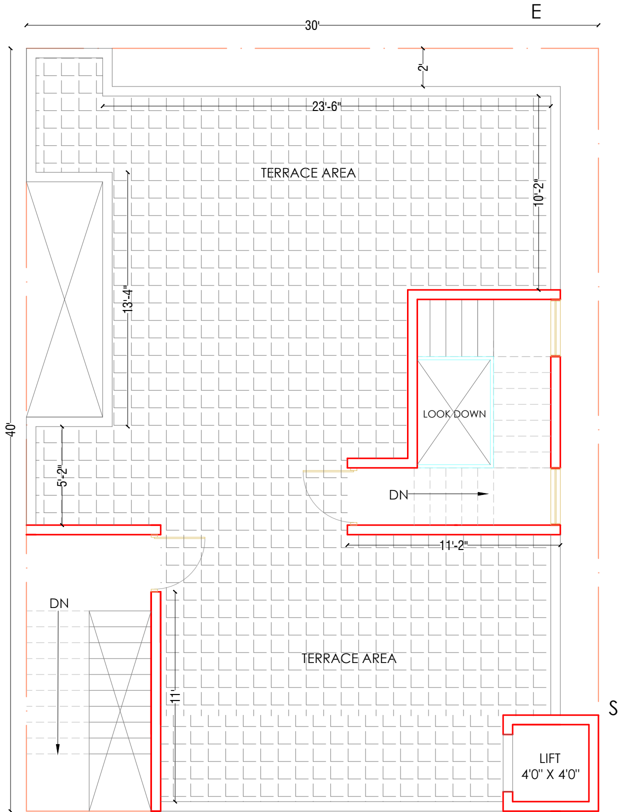
TERRACE FLOOR PLAN:- 246 SFT
